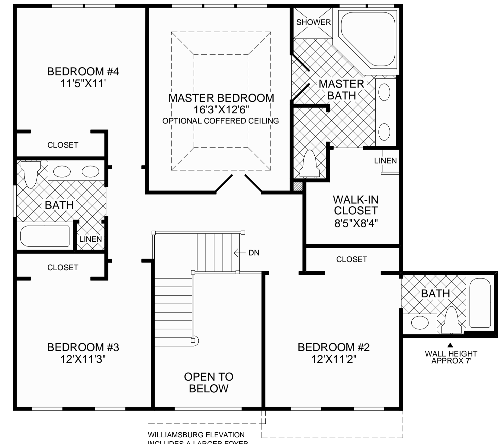
SECOND FLOOR
