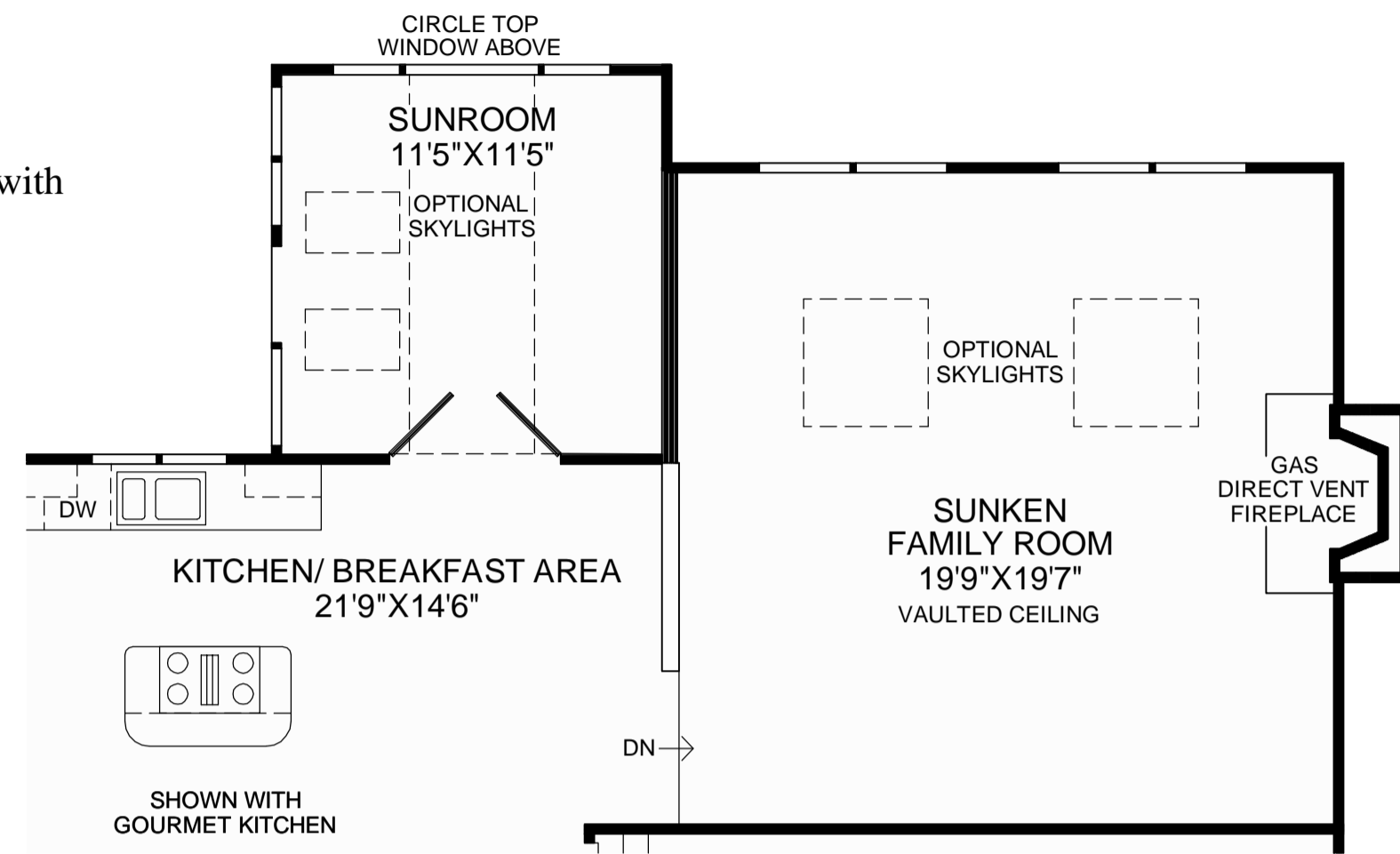
OPTIONAL SARASOTA SUNROOM WITH EXPANDED FAMILY ROOM
